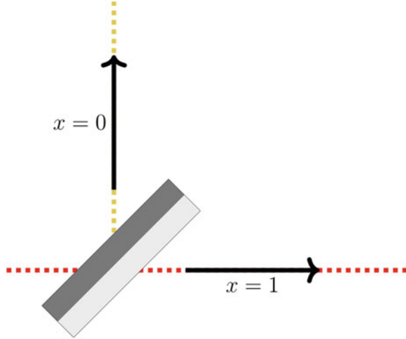
Fig. 9.4 Inputs to the function are photons along two different paths. A photon taking the yellow path is x = 0 , while a photon taking the red path is x = 1 .
