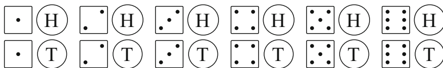
Fig. A.2 All twelve possible outcomes when both rolling a die and flipping a coin
