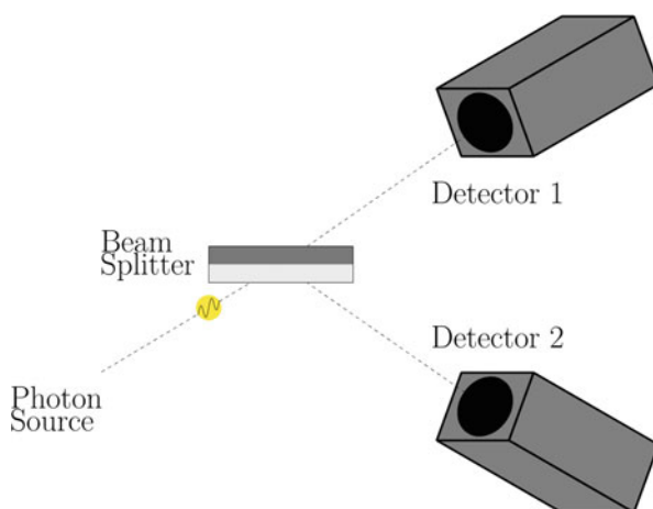
Fig. 3.4 A single photon is sent at a beam splitter and the outcome is measured with detectors to see whether the beam splitter transmits or reflects.
